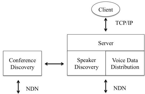
Figure 2: An Overview of ACT Design
