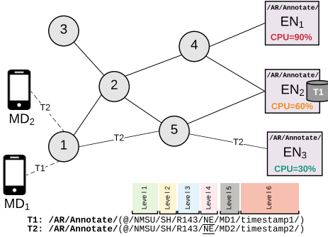
Fig. 2. Scenario highlighting a potential compute reuse if T_2 can be routed to edge node EN_2
