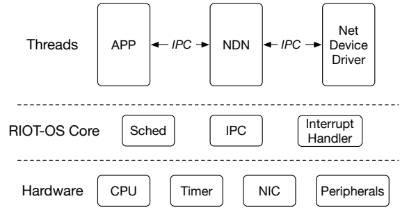
Fig. 1: Software architecture of NDN-RIOT
