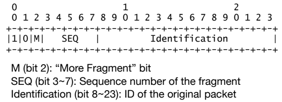
Fig. 2: L2 fragmentation header in NDN-RIOT
